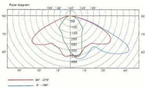
Polar diagram Intensity [cd/1000lm]
